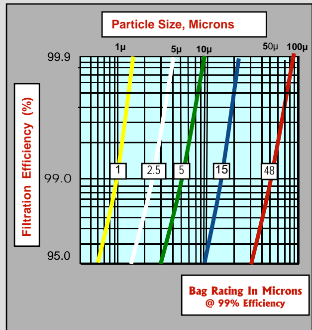
EFFICIENCY CURVES
